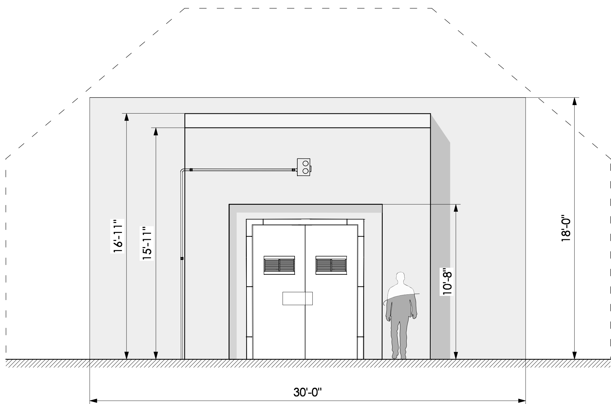
ELEVATION C-C PARTIAL EXTERIOR ENTRANCE
