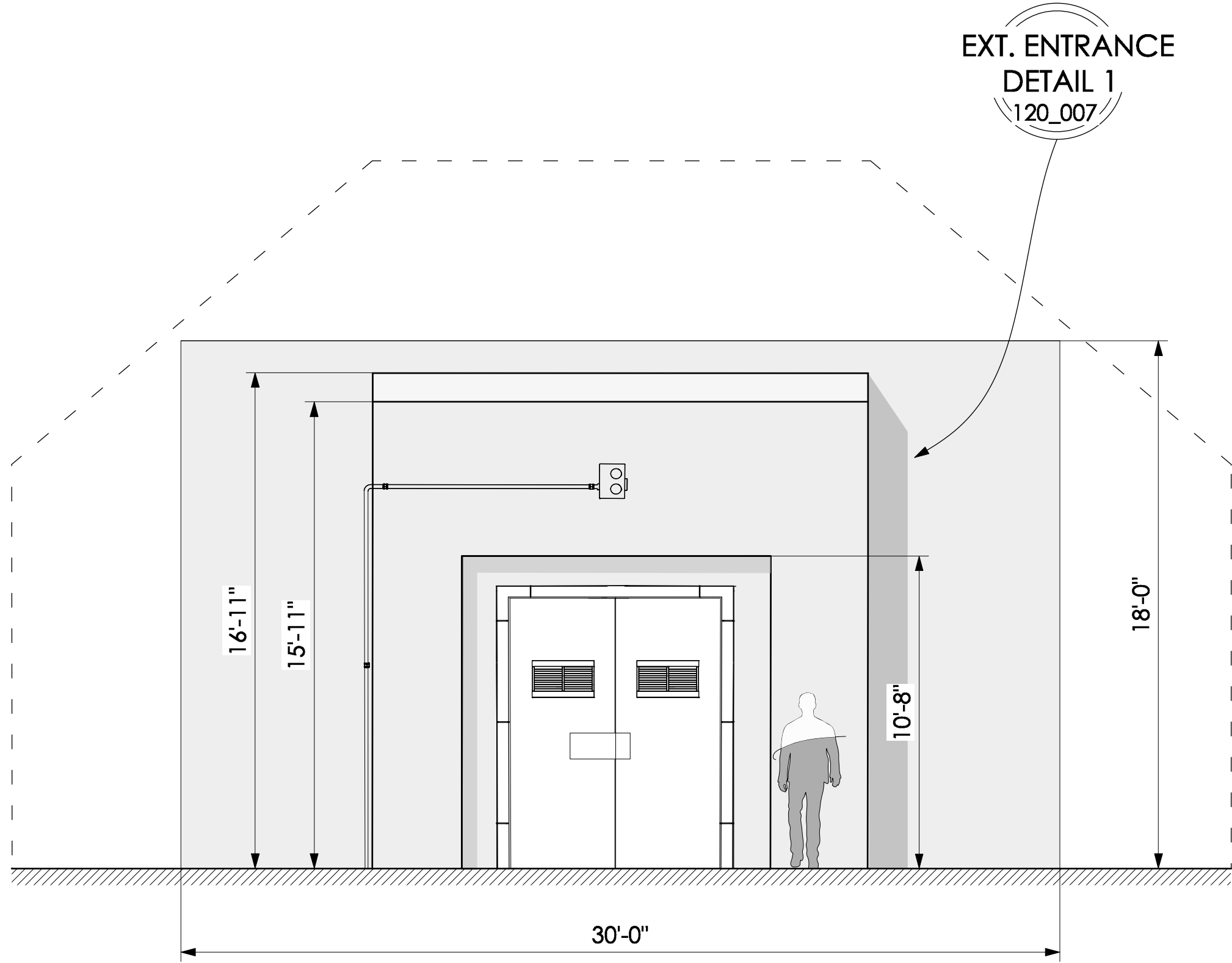
ELEVATION C-C PARTIAL EXTERIOR ENTRANCE
